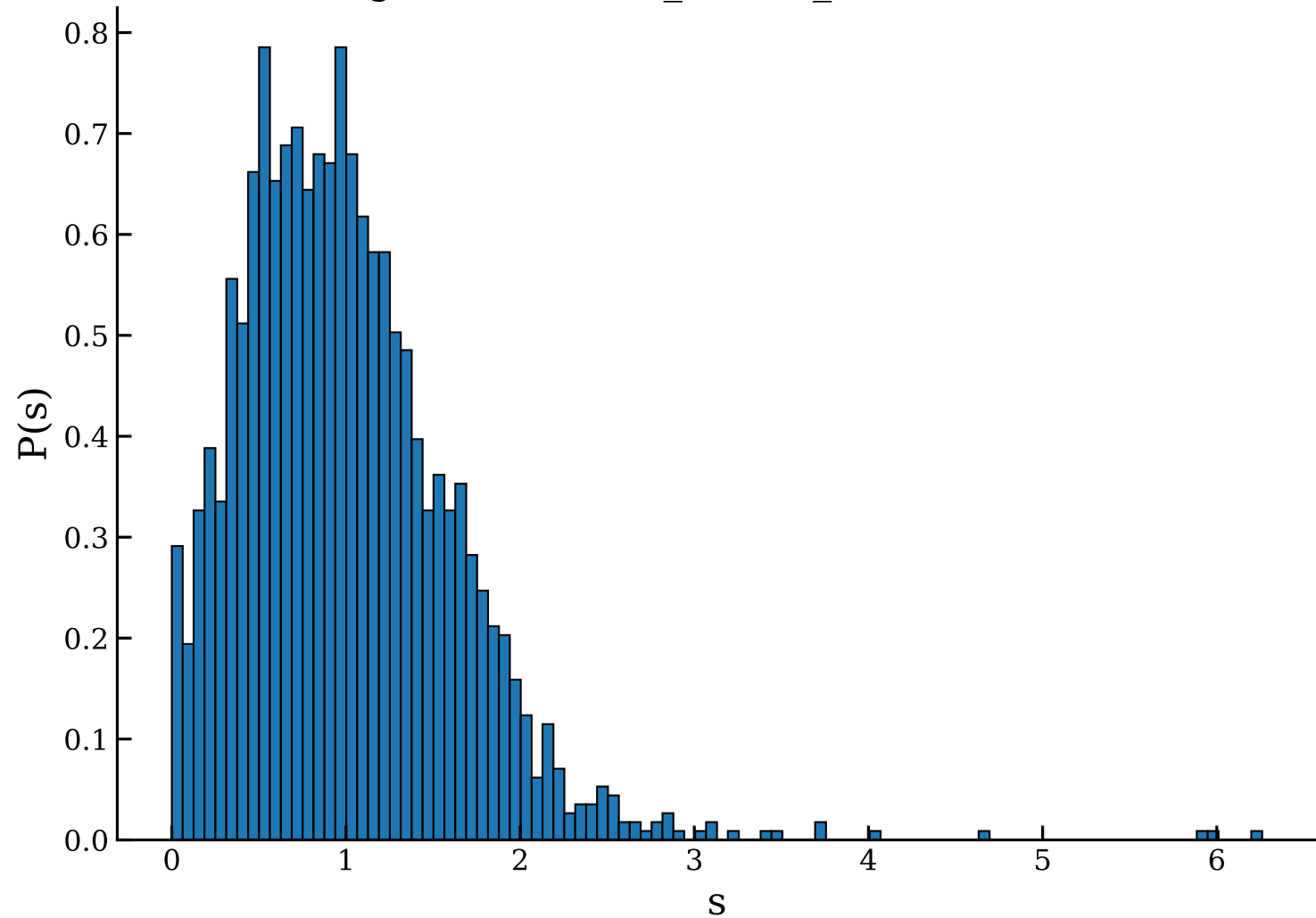
configuration model_N2000_G3 \langle r \rangle = 0.5240
